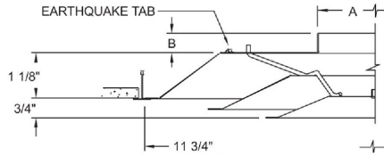
FRAME 22, SURFACE MOUNT, 12" x 12"
