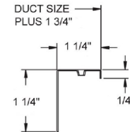
STANDARD FRAME
