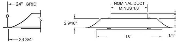
FRAME 23, LAY-IN, T-BAR, 24" x 24" / PLQ SIDE VIEW
