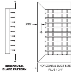
SIDE VIEW AND FACE VIEW
