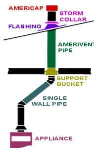
SINGLE INSTALLATION
