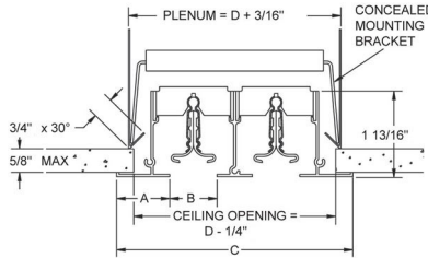
FRAME CROSS SECTION
