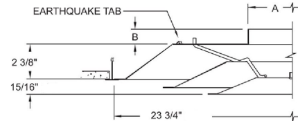
FRAME 23, LAY-IN, T-BAR, 24" x 24"
