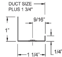
STANDARD FRAME
