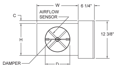
BASE UNIT INLET VIEW
