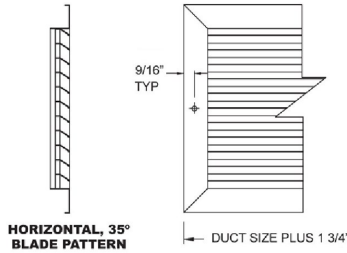
SIDE VIEW AND FACE VIEW
