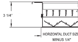
CROSS SECTION
