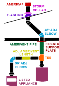
MULTIPLE INSTALLATION
