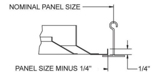
FRAME 23, LAY-IN, T-BAR
