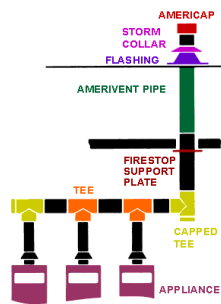
TYPICAL INSTALLATION
