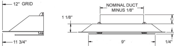
FRAME 23, LAY-IN, T-BAR, 12" x 12" / PLQ SIDE VIEW
