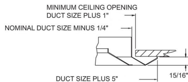
FRAME 21, SURFACE MOUNT, BEVELED
