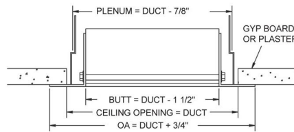
FRAME SIDE VIEW
