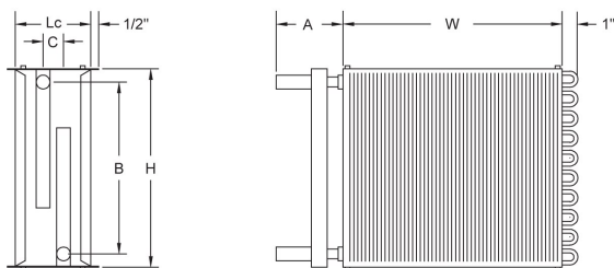
2 ROW HOT WATER COIL SIDE VIEW/FACE VIEW
