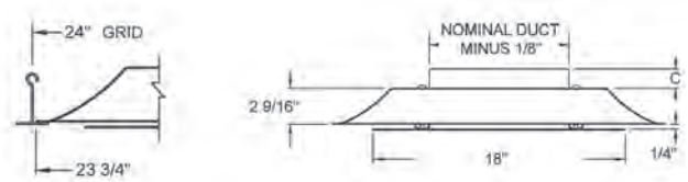
FRAME 23, LAY-IN, T-BAR, 24" x 24" / PLQ SIDE VIEW
