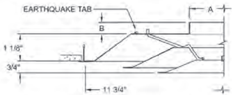
FRAME 22, SURFACE MOUNT, 12" x 12"
