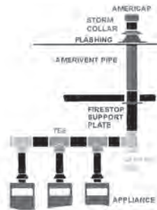
TYPICAL INSTALLATION
