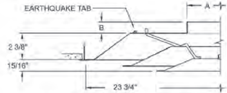
FRAME 23, LAY-IN, T-BAR, 24" x 24"
