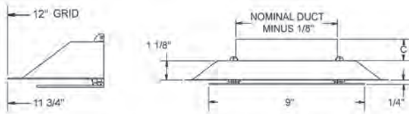
FRAME 23, LAY-IN, T-BAR, 12" x 12" / PLQ SIDE VIEW
