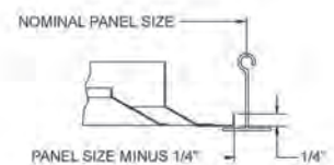
FRAME 23, LAY-IN, T-BAR
