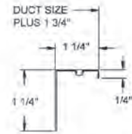
STANDARD FRAME
