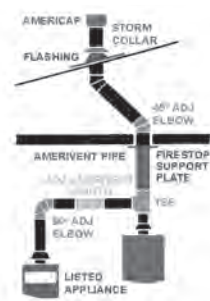
MULTIPLE INSTALLATION
