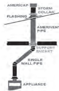
SINGLE INSTALLATION
